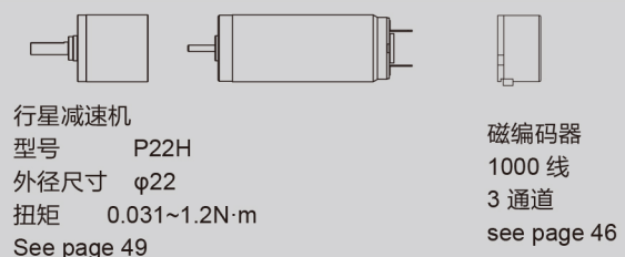
SMJ配件 SMJ Modular System
